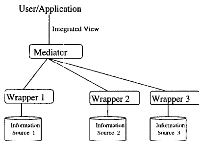
Figure 1: The TSIMMIS integration architecture
