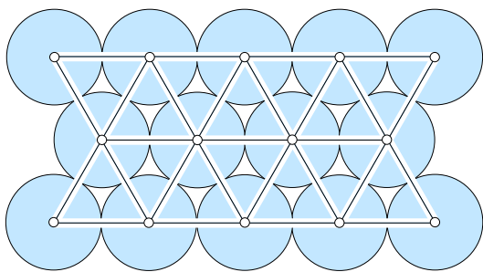
Figure 3: Portion of a densest packing of disks in the plane.
