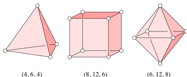
Figure 1: Three of the five Platonic solids together with their face vectors. From left to right: the tetrahedron, the cube, and the octahedron.
