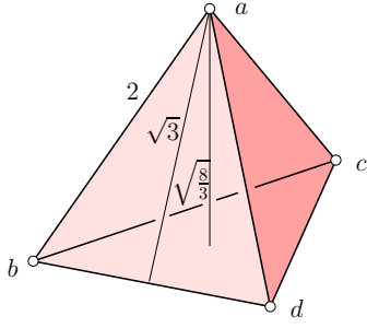
Figure 5: A regular tetrahedron with edges of length 2 has height \sqrt{8/3} . Its four triangles have height \sqrt{3} each.
