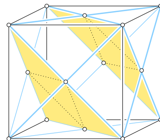
Figure 4: We have a sphere centered at each vertex and at the center of each face of the cube.
