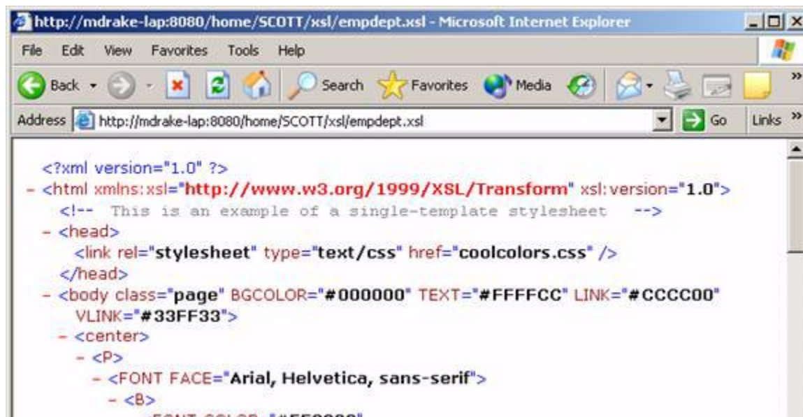
Figure 26–52 XSL Style Sheet for Use with DEPTVIEW
