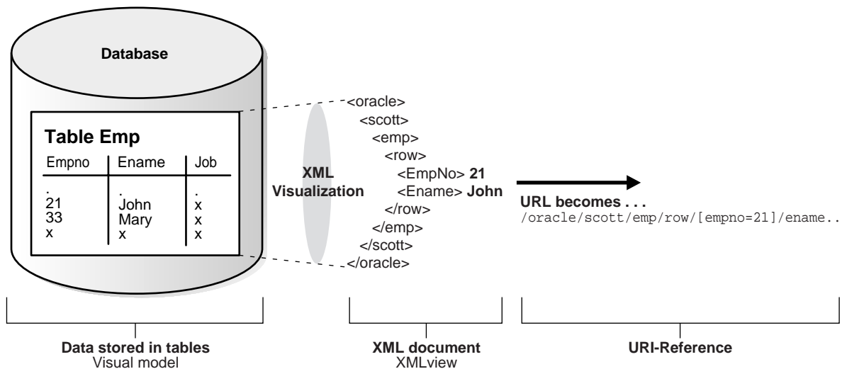
Figure 12–1 DBUri: Visual or SQL View, XML View, and Associated XPath
