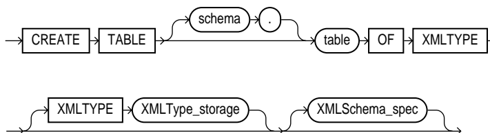
Figure 5-1 Creating an XMLType Table
