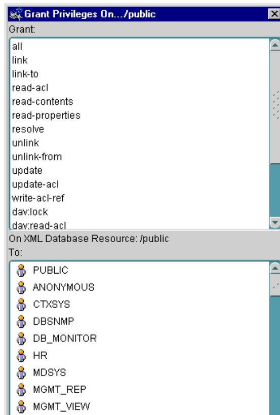
Figure 21–11 Enterprise Manager: Granting Privileges On Oracle XML DB Resources
