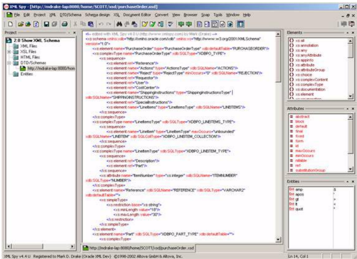
Figure 26–12 XML Schema Displayed in Native Form, an XML Document
