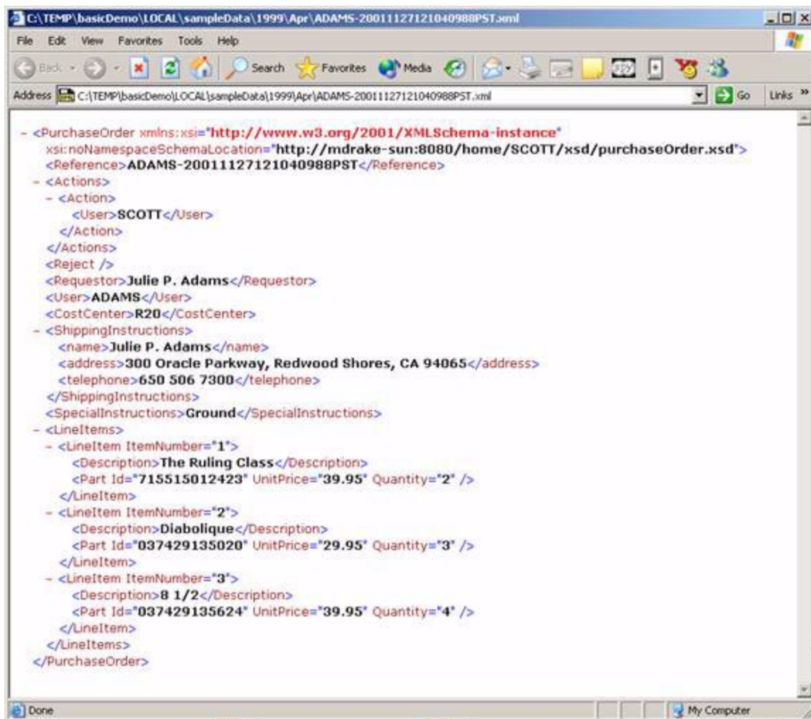
Figure 26–16 Displaying Document ADAMS-2011127121040988PST.xml
