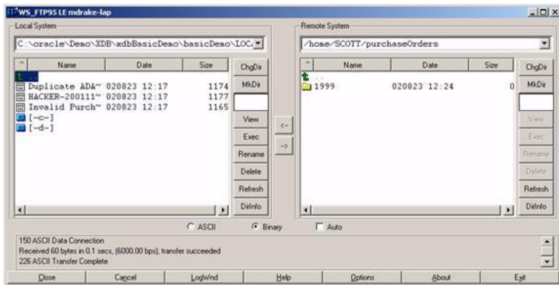
Figure 26–19 Opening the FTP Client to Establish an FTP Connection
