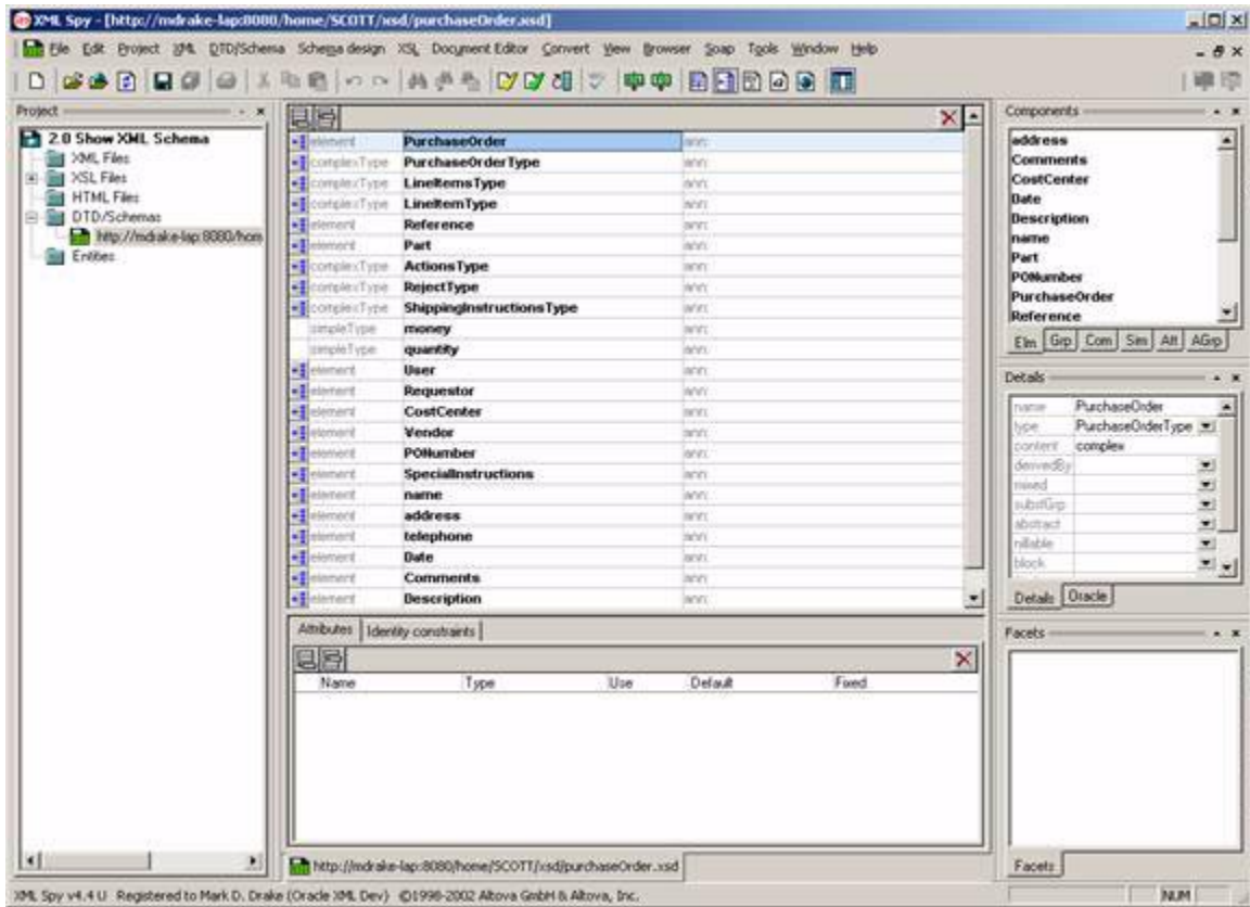
Figure 26–10 XMLSpy's Graphical Representation of Elements and Types Defined by the XML Schema
