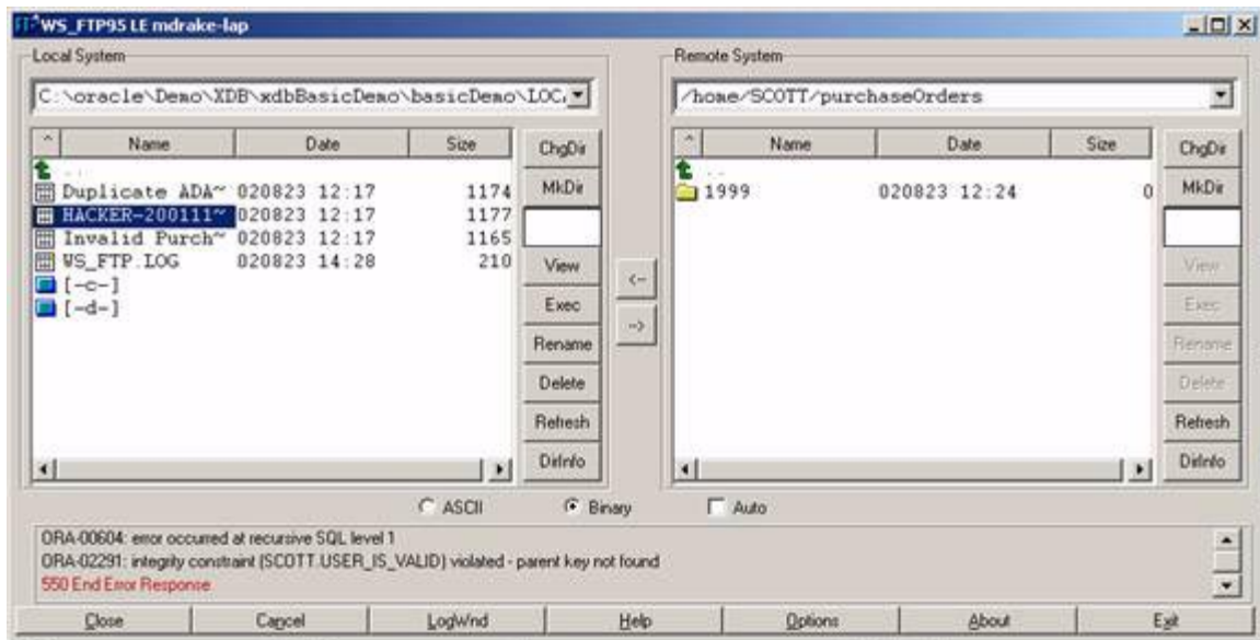
Figure 26–21 FTP Error Caused From Violating the USER_IS_VALID Constraint
