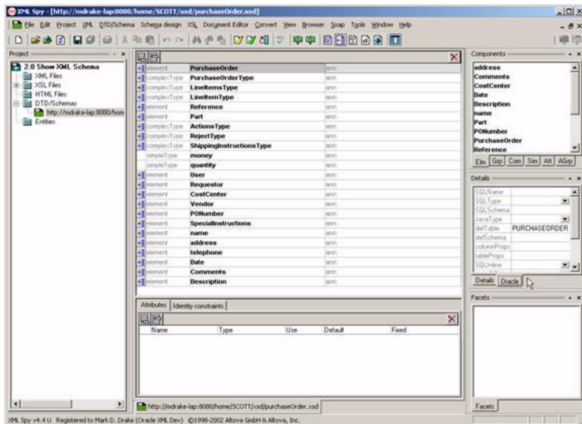
Figure 26–13 A Graphical View of XML Schema
