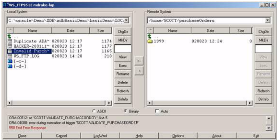
Figure 26–22 FTP Error Caused From Firing the VALIDATE_PURCHASEORDER Trigger
