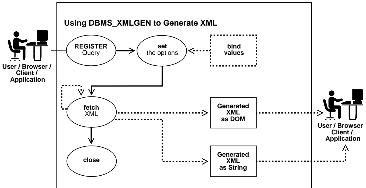
Figure 10–9 DBMS_XMLGEN Calling Sequence
