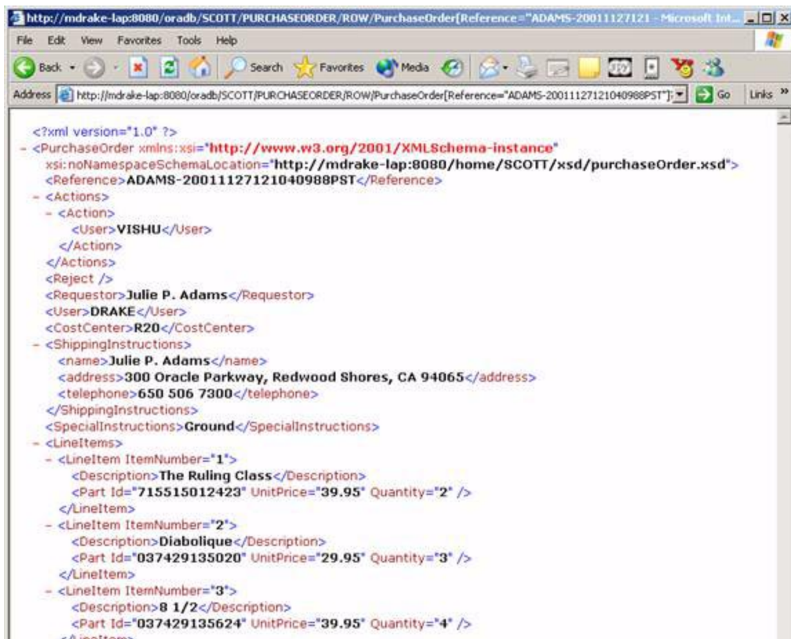
Figure 26–47 Using DBUriServlet and DBUriType to Select Rows from an XML Document, Based on a URL.
