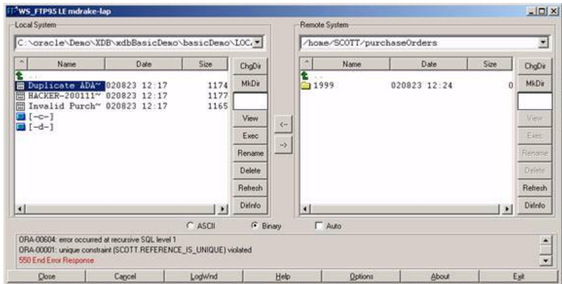
Figure 26–20 FTP Error Caused From Violating the UNIQUE Constraint
