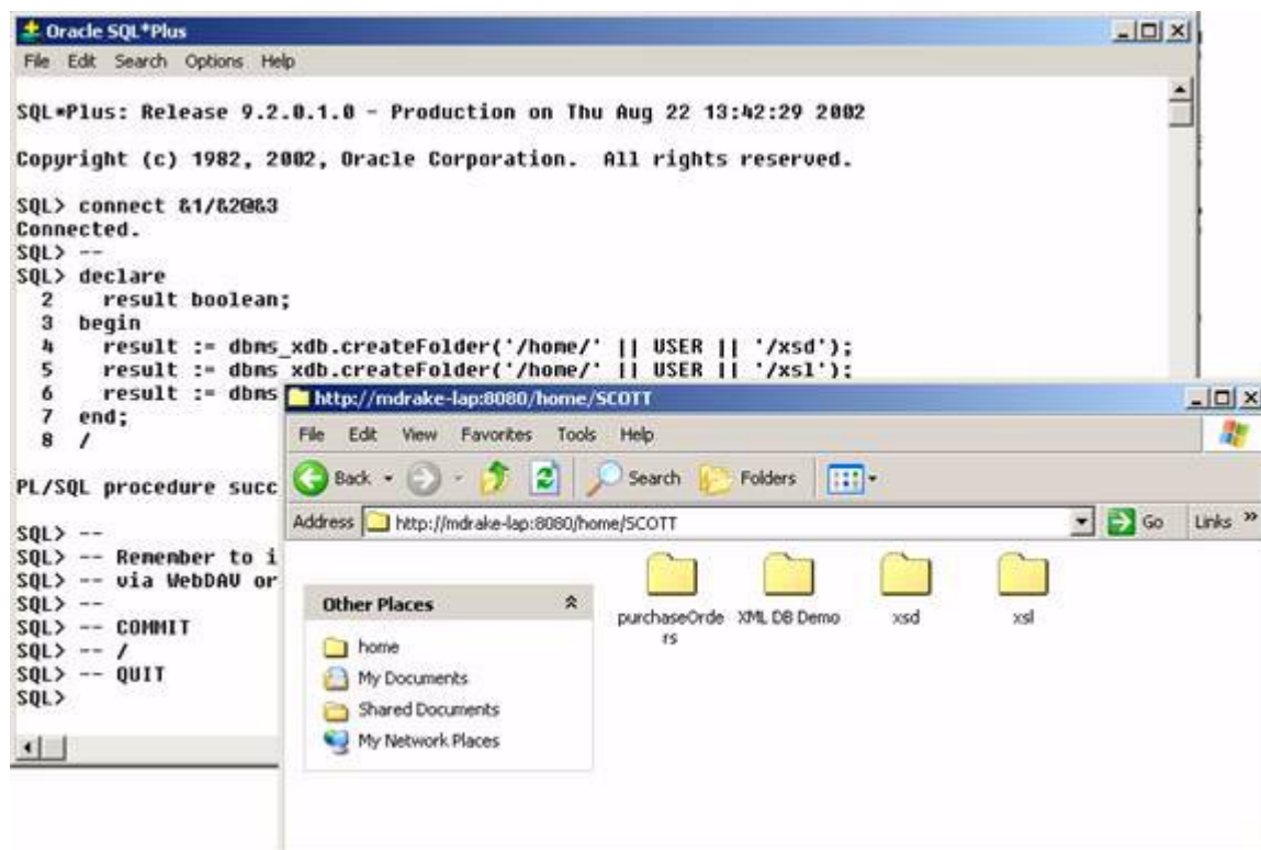
Figure 26–7 Executing the PL/SQL Script: Folders are Visible
