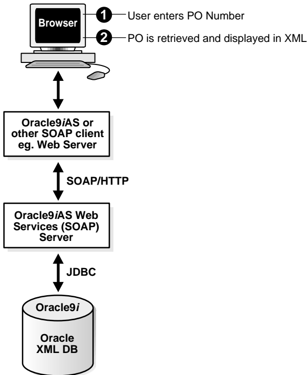
Figure 25–2 XML DB Web Services Case Study: Main Components
