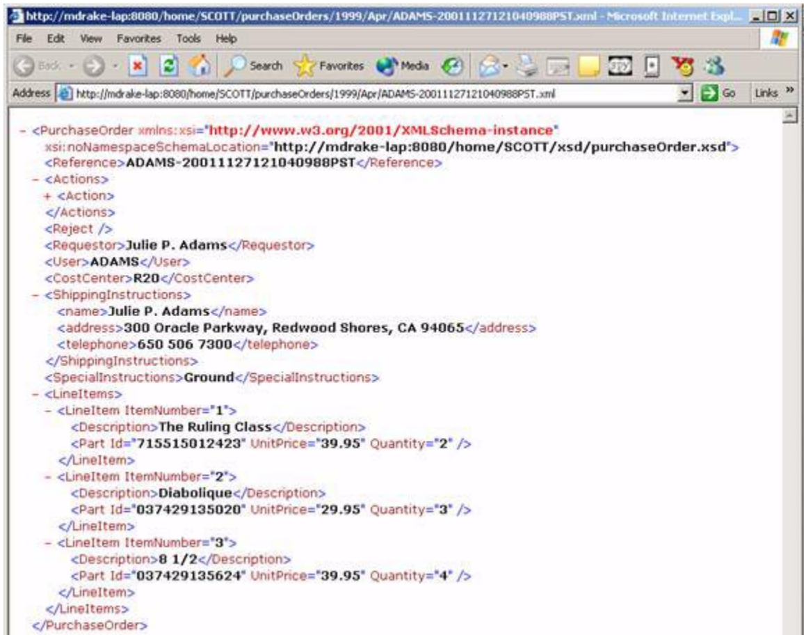
Figure 26–30 PurchaseOrder XML Document is Displayed
