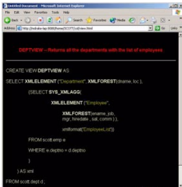
Figure 26–50 HTML Page Showing XMLType View DEPTVIEW
