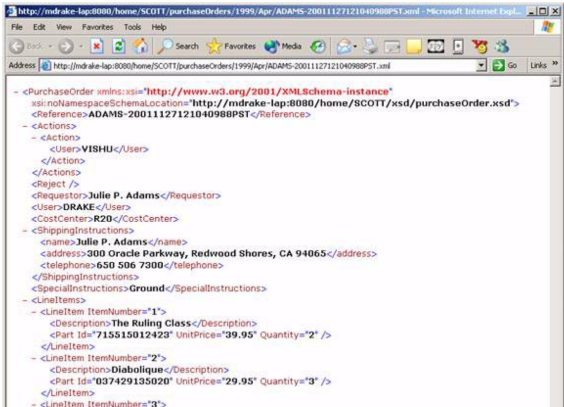
Figure 26–35 Interoperability of XML and SQL: Accessing XML Content Using SQL
