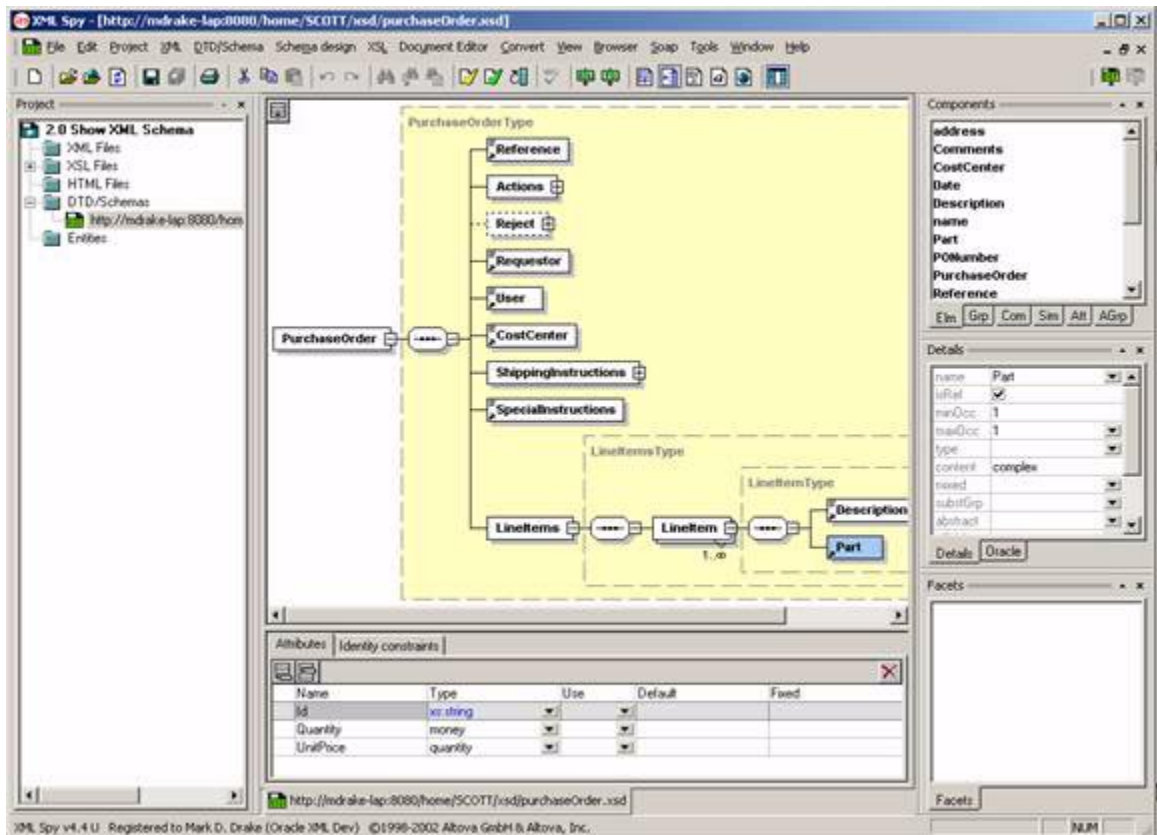
Figure 26–11 XMLSpy Displays the PurchaseOrder XML Schema
