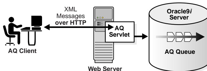
Figure 24–2 IDAP Architecture for Performing AQ Operations Using HTTP
