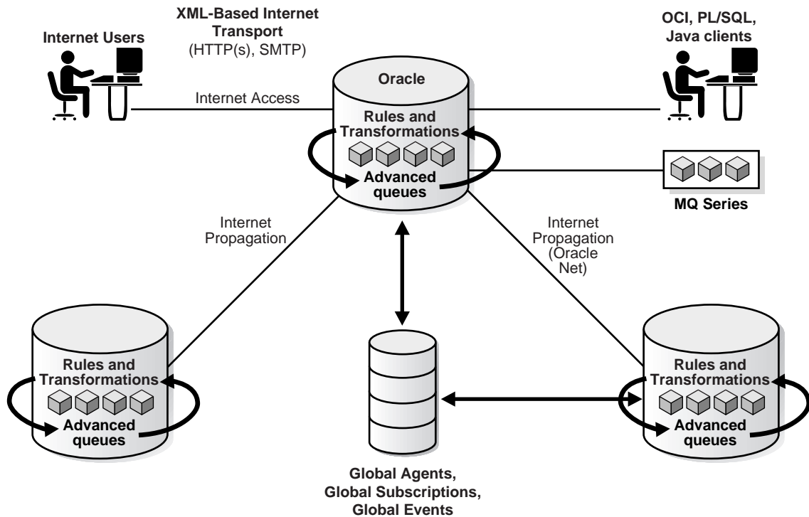
Figure 24–1 Advanced Queuing and XML Message Payloads
