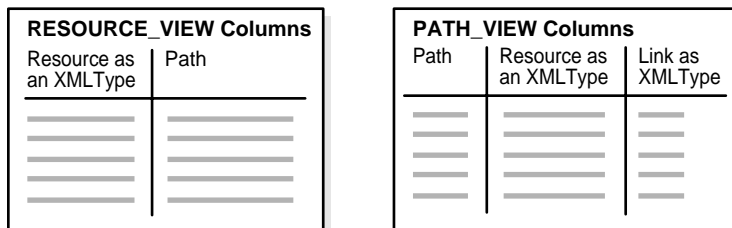
Figure 15-2 RESOURCE_VIEW and PATH_VIEW Structure
