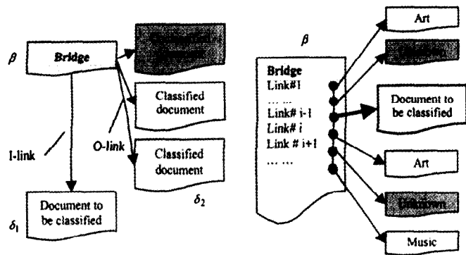
Figure 8: The phenomenon of pages that bridge topics across length-two paths. The second diagram shows how one may try to exploit locality in the topics on bridge pages.
